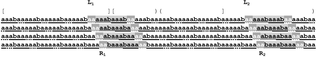
Figure 1: Cyclic shifts of the inversion factor and its environment
