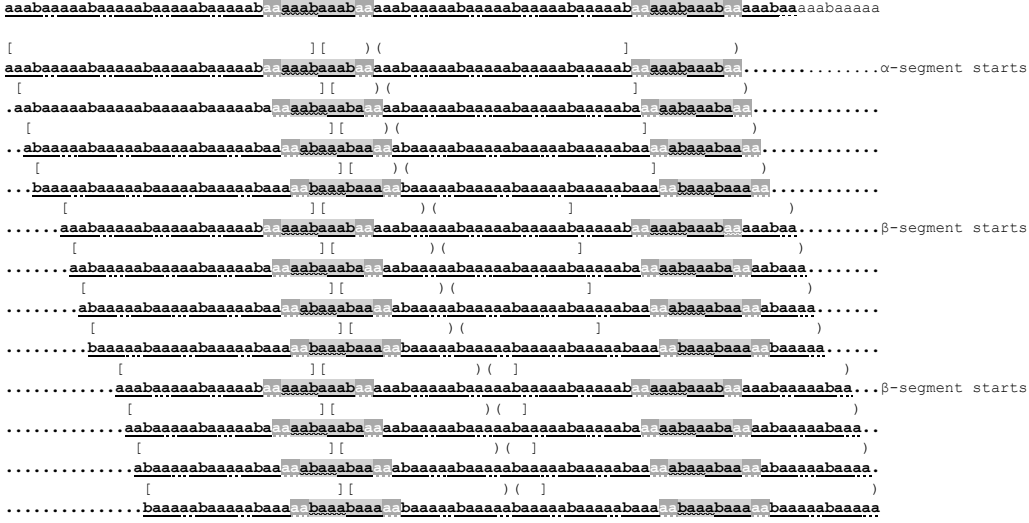
Figure 4: Example of an (\alpha+\beta) -family of \mathcal{U}
