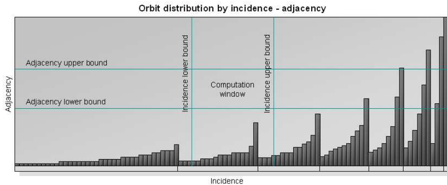
Figure 4.2: Computation window
