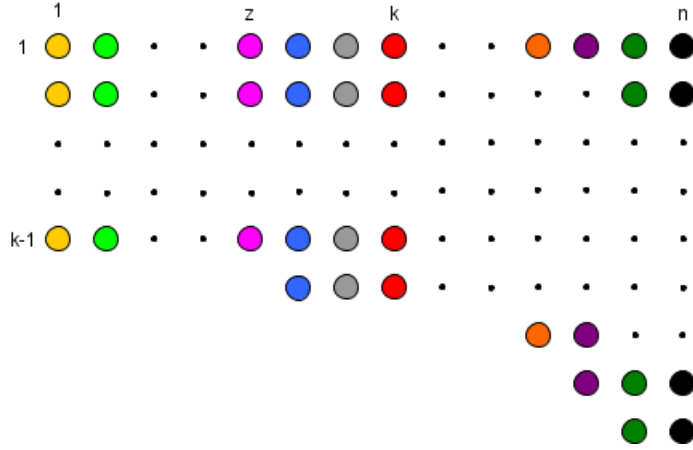
FIGURE 4. The vertex set of the (k-1, \dots, k-1, k, \dots, k, m_{k+1}, \dots, m_n) -octahedral system \Omega = (V_1, \dots, V_n, E) used for the proof of Proposition 4.5
