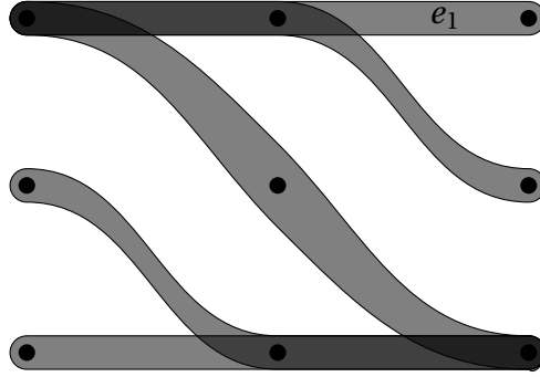
FIGURE 1. \Omega^{(3,3)} : a (3,3,3) -octahedral system matching the upper bound given in Proposition 2.4
