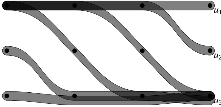
FIGURE 2. \Omega^{(3,4)} : a (3,3,3,3) -octahedral system matching the upper bound given in Proposition 2.4
