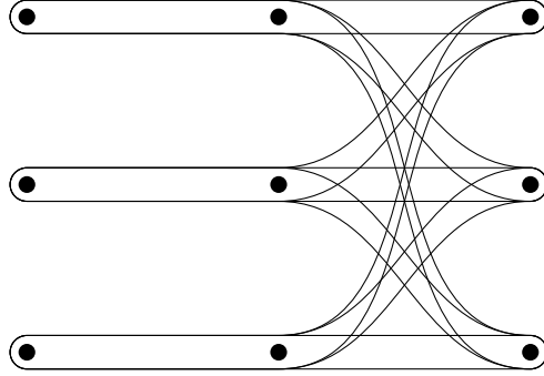
FIGURE 3. A non realisable (3,3,3)-octahedral system with 9 edges
